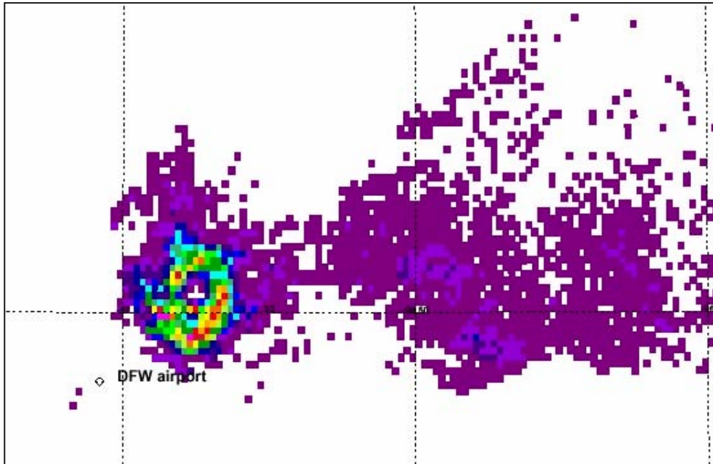
Figure 1. VHF source density (src/km 2 ) on 1X1 km 2 grid for 04:04-04:07 UTC on April 6, 2003. Each color change represents an additional 10 src/km 2 .
